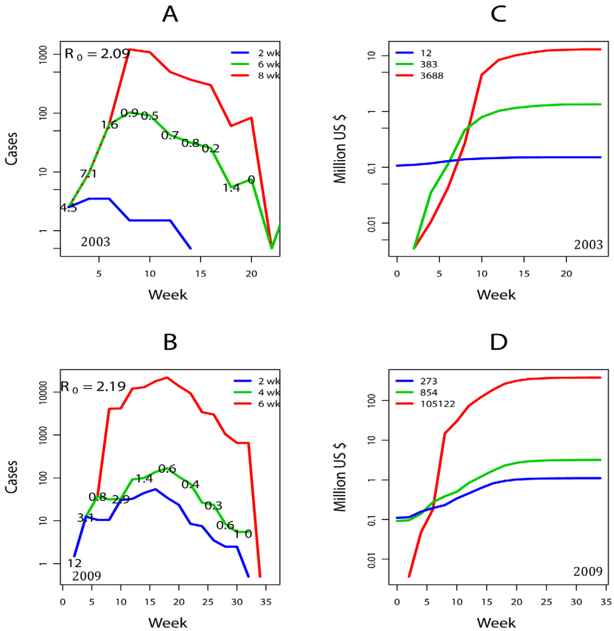
Figure 1. Impacts of hypothetical scenarios of delayed response of vector control to Dengue virus outbreaks. The basic reproduction number, R_0 (the average number of secondary cases after the introduction of an infection) for the 2003 and 2009 dengue fever outbreaks that affected the city of Cairns, Australia, was estimated by fitting an exponential function to the observed weekly epidemic curves before vector control interventions began (6 weeks in 2003 and 4 weeks in 2009). The effective reproduction number, R_t (the average number of secondary cases per primary case at time t ) of each outbreak was estimated by accumulating the number of cases in biweekly periods (the average generation time of dengue is \sim 14 days) and computing the ratio between consecutive two-week periods. The hypothetical epidemic curves for the 2003 (A) and 2009 (B) outbreaks under different scenarios for response times ( res ) of vector control activities to a dengue introduction ( res = 2, 4, 6 and 8 weeks) were computed by estimating the number of cases in the absence of control (between t_0 and res ) using R_0 , and then generating the rest of each epidemic time series by multiplying the number of cases by the estimated post intervention R_t in the original series. Blue lines indicate a faster response time than in the actual outbreak, red lines indicate scenarios where the response is delayed in comparison to the actual outbreak, and green lines indicate the actual outbreak. Values on top of the green lines are estimates for R_t . Cumulative cost (in 2009 US$) of each res scenario were estimated for the 2003 (C) and 2009 (D) outbreaks. Figure legends refer to each res scenario (A,B) and to the final epidemic size of each scenario (C,D). doi:10.1371/journal.pntd.0000858.g001
