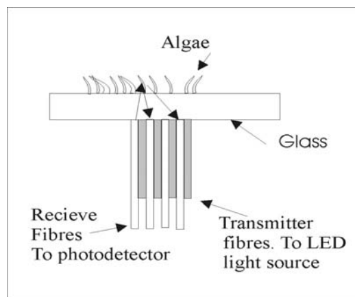
Figure 5.1: Principle of operation of sensor. Light from a bundle of optic fibres illuminates the algae on a glass plate. Fluorescent emissions from the algae are detected by a photodetector at the end of a second bundle of fibre.
