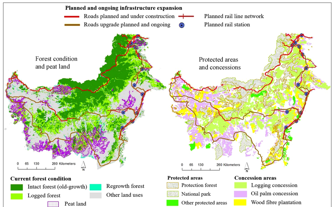
Figure 4. Planned and ongoing infrastructure-expansion routes with respect to current forest condition, peatland, protected areas, and concessions in Indonesian Borneo. In the figure, other protected areas include nature reserves, wildlife reserves, sanctuary reserves, citizen forestry parks, and nature recreation parks that each comprise less than 5% of all protected areas. The maps were created using Esri ArcMap 10.4.1 ( https://www.arcgis.com ).
